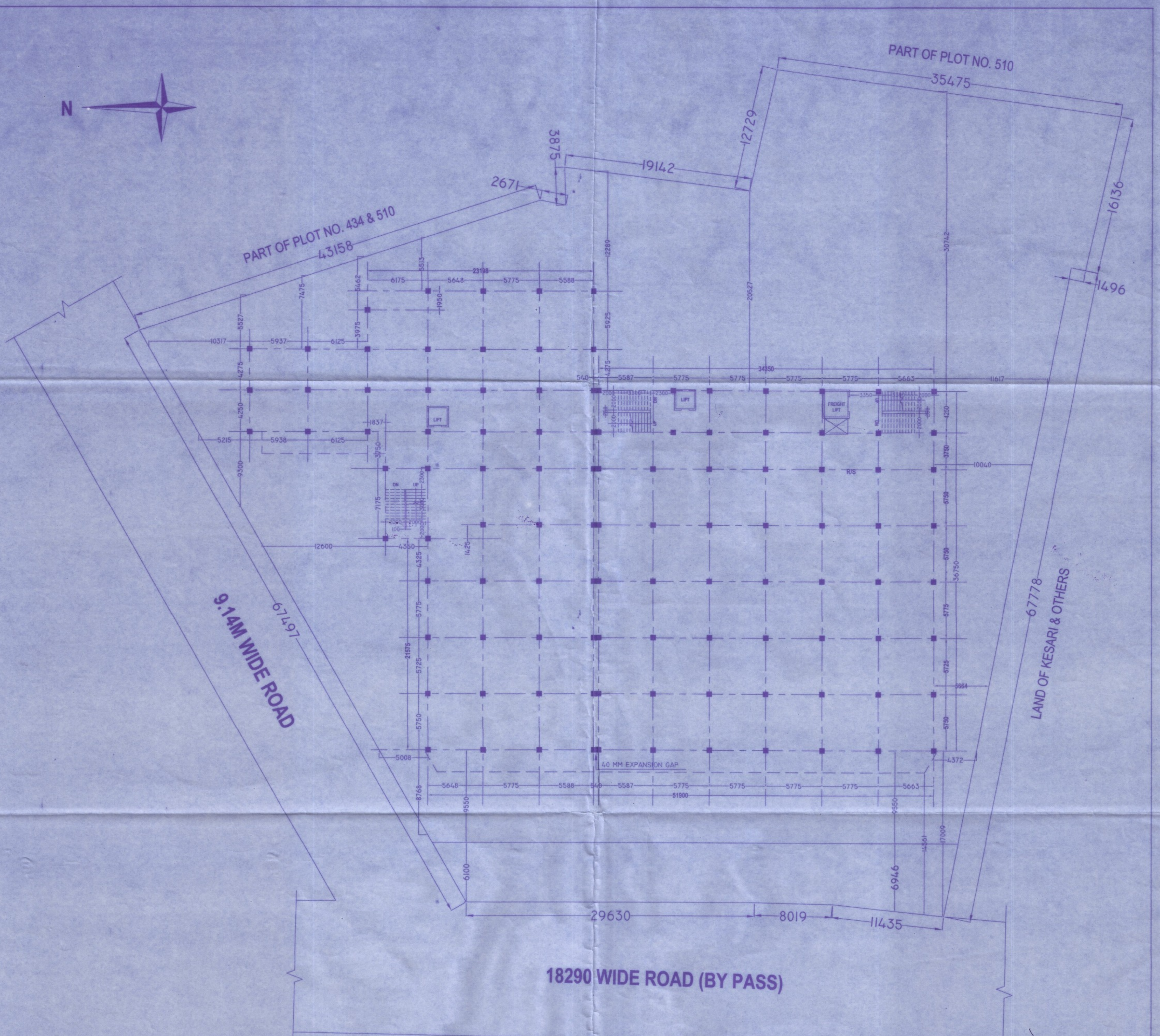
COLUMN LAYOUT PLAN SCALE - 1 : 200
